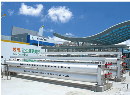
Skid-mounted Hydrogen Refueling Station
